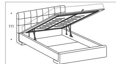
Ring "PRS/B" (slats included)
